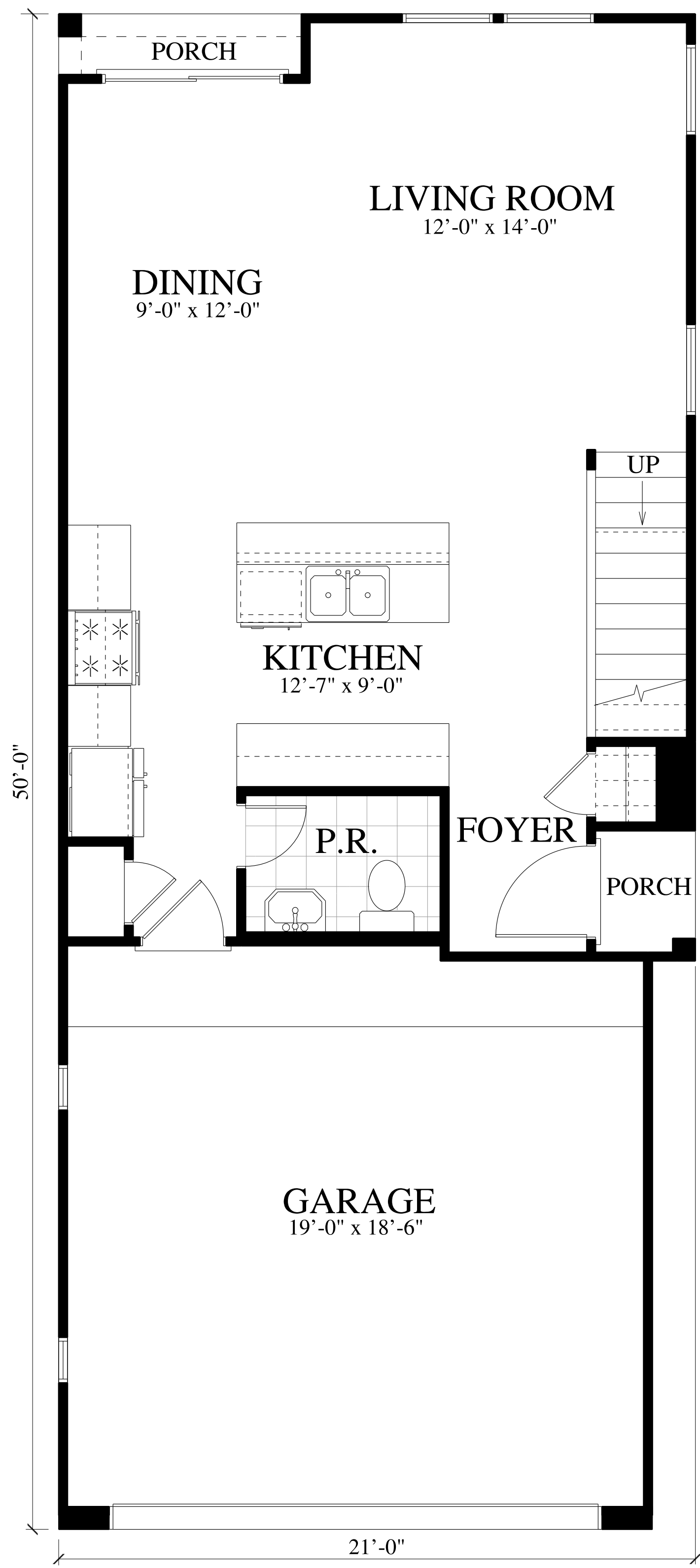
FIRST FLOOR PLAN 620 S.F.
